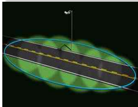
Wide angle optics distribution
